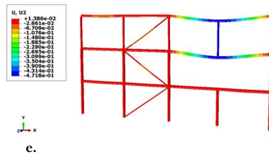
Fig. 19. Outputs from the analysis in the eighth state; a. Strain, b. Column axial force, c. Tension, d. Column removal location relocation history, and e. Modified frame shape.
