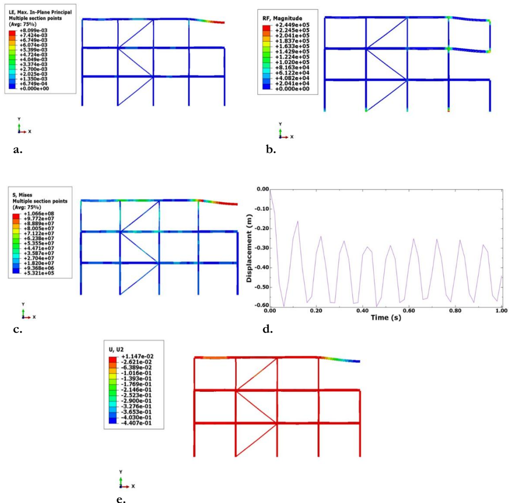
Fig. 16. Outputs from the analysis in the fifth case; a. Strain, b. Column axial force, c. Tension, d. Column removal location relocation history, and e. Modified frame shape.
