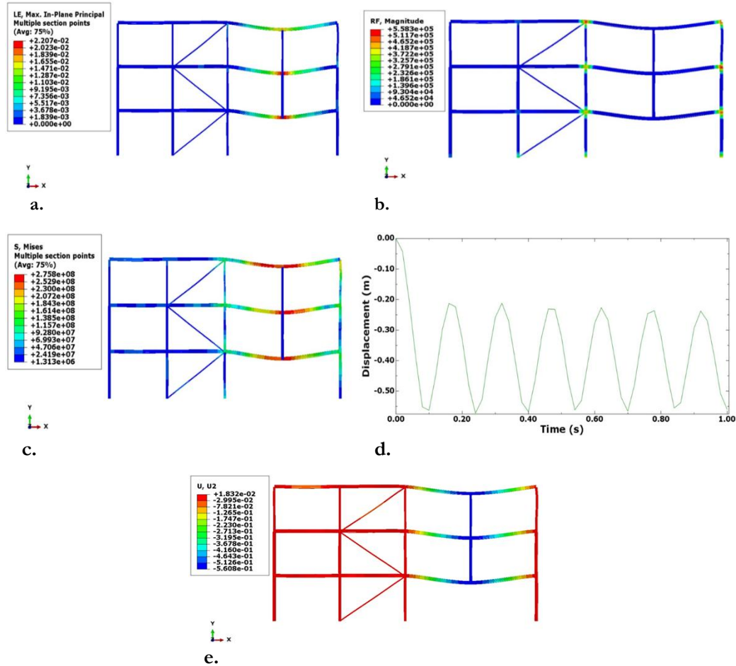
Fig. 17. Outputs from the analysis in the sixth state; a. Strain, b. Column axial force, c. Tension, and e. Modified frame shape.
