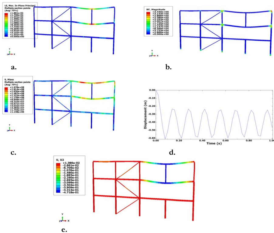
Fig. 18. Outputs from the analysis in the seventh state; a. Strain, b. Column axial force, c. Tension, d. Column removal location relocation history, and e. Modified frame shape.
