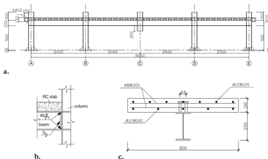
Fig. 1. Frame details and dimensions; a. detail dimension of frame (mm), b. full-welded beam-to-column connection, and c. cross section composite beam.
