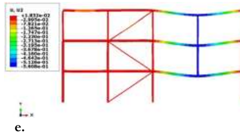
Fig. 17. Outputs from the analysis in the sixth state; a. Strain, b. Column axial force, c. Tension, e. Modified frame shape.
