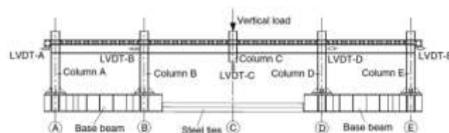
Fig. 4. Distribution of displacement gauges in different parts of the frame.
