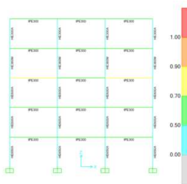
Fig. 3. Stress ratio in elements in a 5-story frame.
