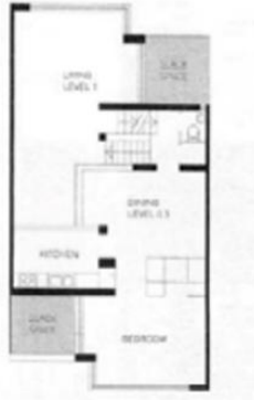
Horizontal expansion in defined space; the potential for growth is provided horizontally Diagoon Houses, Netherlands, 1971 Architect: Herman Hertzberger First Floor Plan
