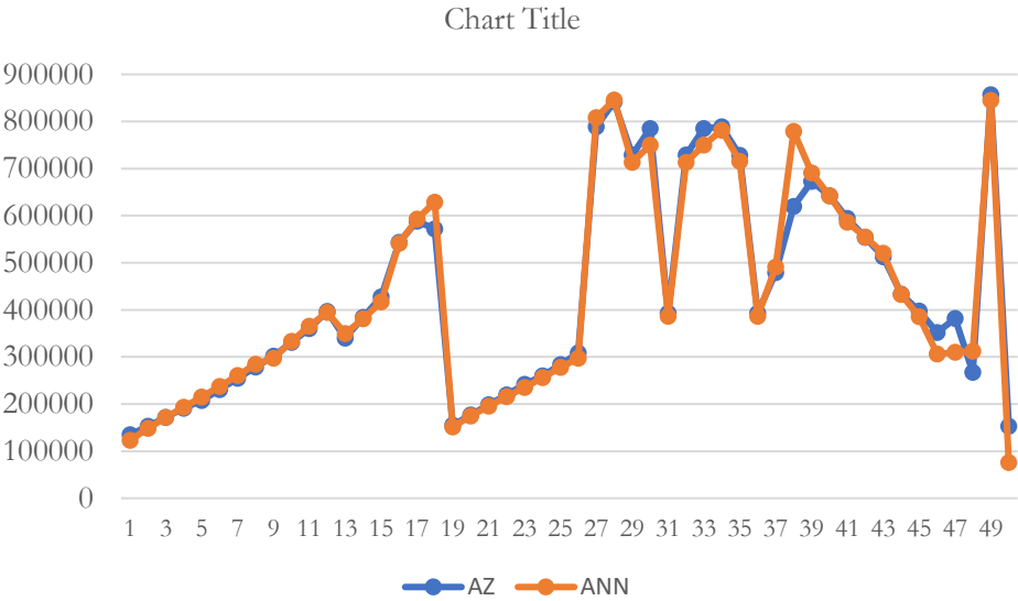
Fig. 5. Comparison of pile bearing capacity results with neural network and laboratory data.
